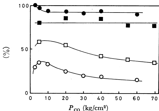
Fig. 2. Effect of the pressure of CO. ○ (Conv.) and ● (Select.) under the condition that C_6H_5I 40 mmol, C_6H_6 30 ml, MeOH 280 mmol, NEt_3 50 mmol, Pd-black 0.5 mmol, and Time 90 min. □ (Conv.) and ■ (Select.) under the condition that C_6H_5I 40 mmol, MeOH 30 ml, AcOK 50 mmol, Pd-black 0.25 mmol and Time 90 min.
